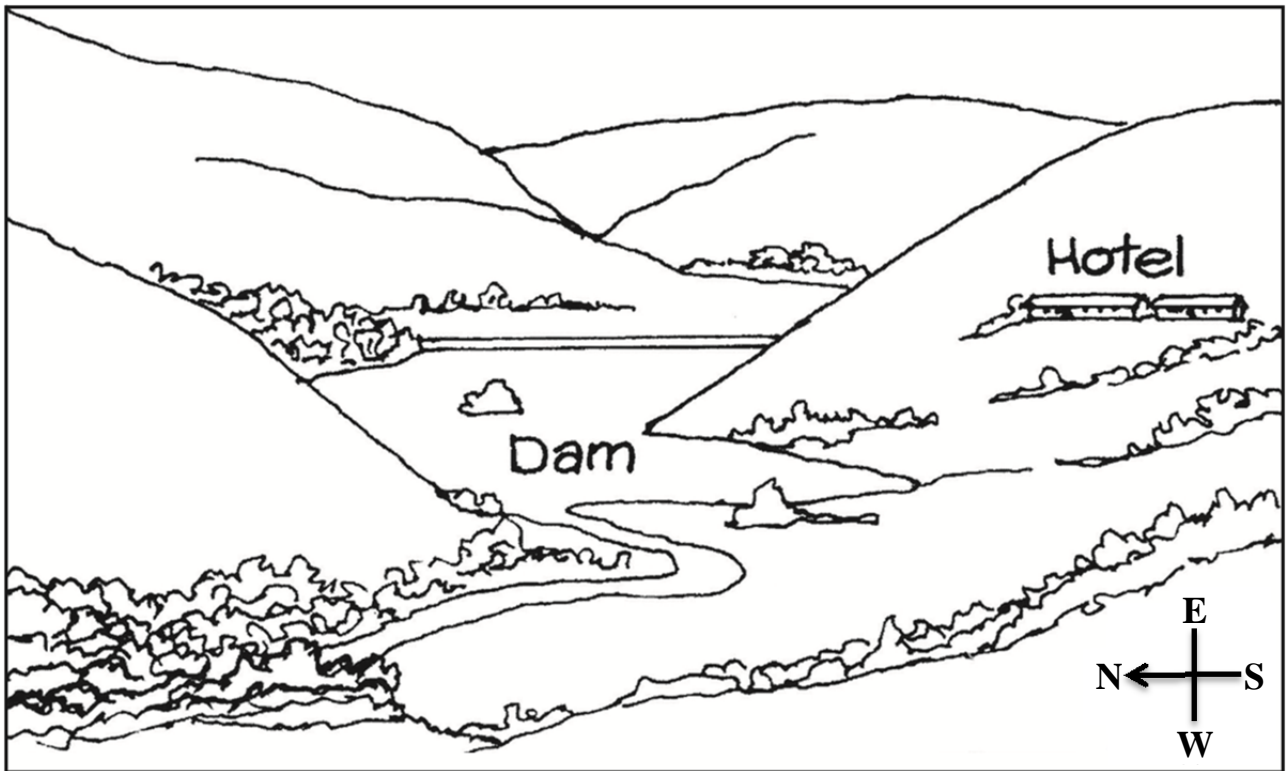
Figure 2: Field sketch of the Drakensberg valley (Photograph 2) – Question 1.1.4 and Question 1.2.1
