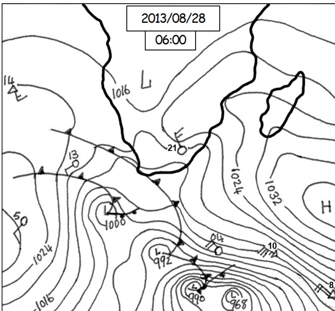
Figure 1: Synoptic weather map for 28 August 2013 – Question 1.1.2 and Question 1.1.3
