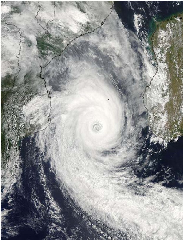
Photograph 3: Satellite image of Funso – Question 2.1
