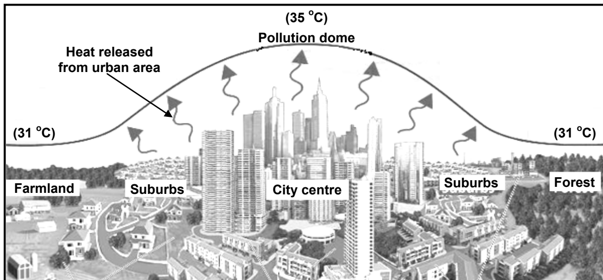
FIGURE 1.3: CITY CLIMATE
