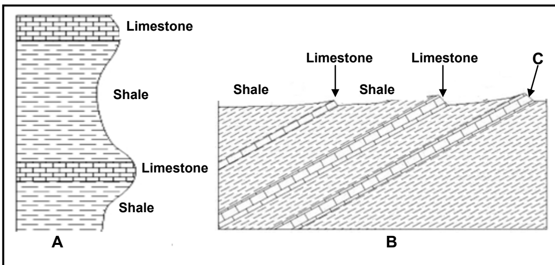
FIGURE 2.2: SEDIMENTARY STRATA/LAYERS
