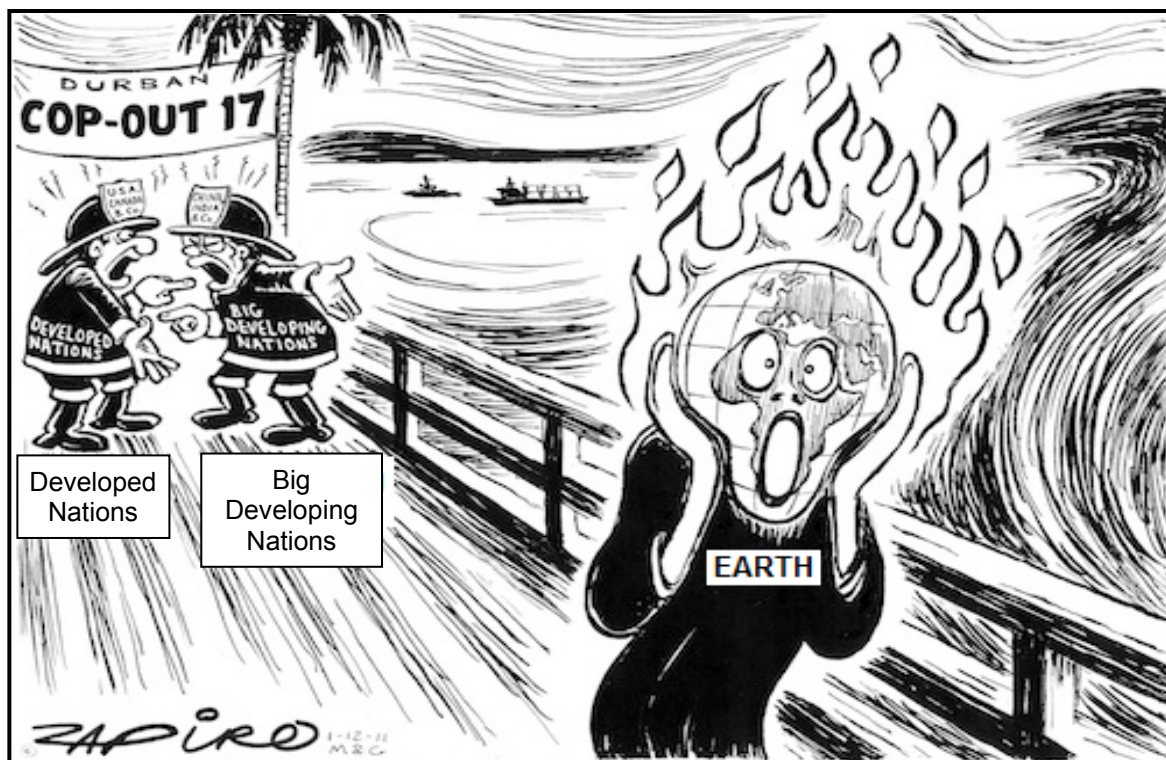
FIGURE 2.4: GLOBAL WARMING
